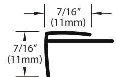
WC-101- Outside Corner
