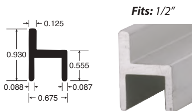
Part # Finish ALU120-S Satin
