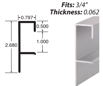
Part # Finish ALU1160-S Satin
