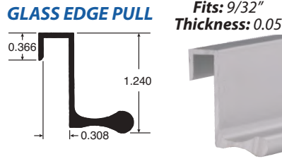
Part # Finish ALU3108-S Satin
