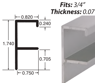
Part # Finish ALU1500H-S Satin
