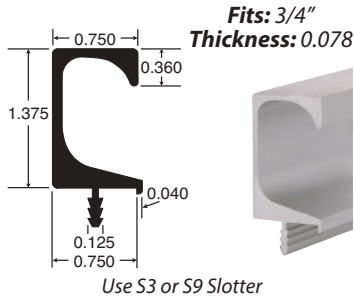
Part # Finish ALU126-S Satin
