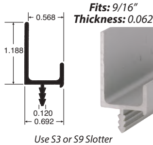
Part # Finish ALU1510-S Satin
