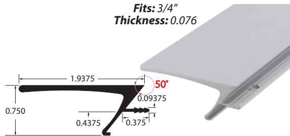
Part # Finish PLX-KL8LA-S Satin
