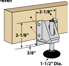
Support Brace With Leveler (adjust with 5mm hex key) Set Includes 1 Brace & 1 Leveler
