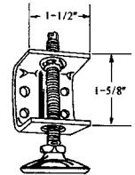
Support Brace With Leveler (adjust with 5mm hex key) Set Includes 1 Brace & 1 Leveler
