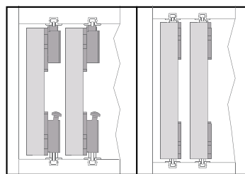
Surface Mount Flush Mount Carrier Installation
