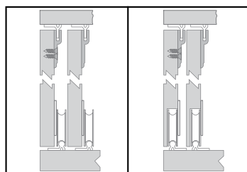
Surface Mount Recessed Mount Carrier Installation
